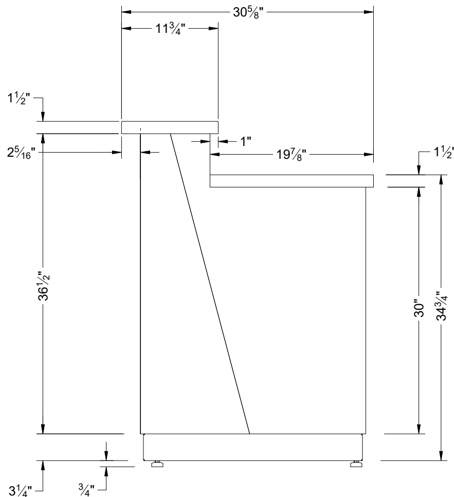
3 ELEVATION 2 SERVICE DESK
