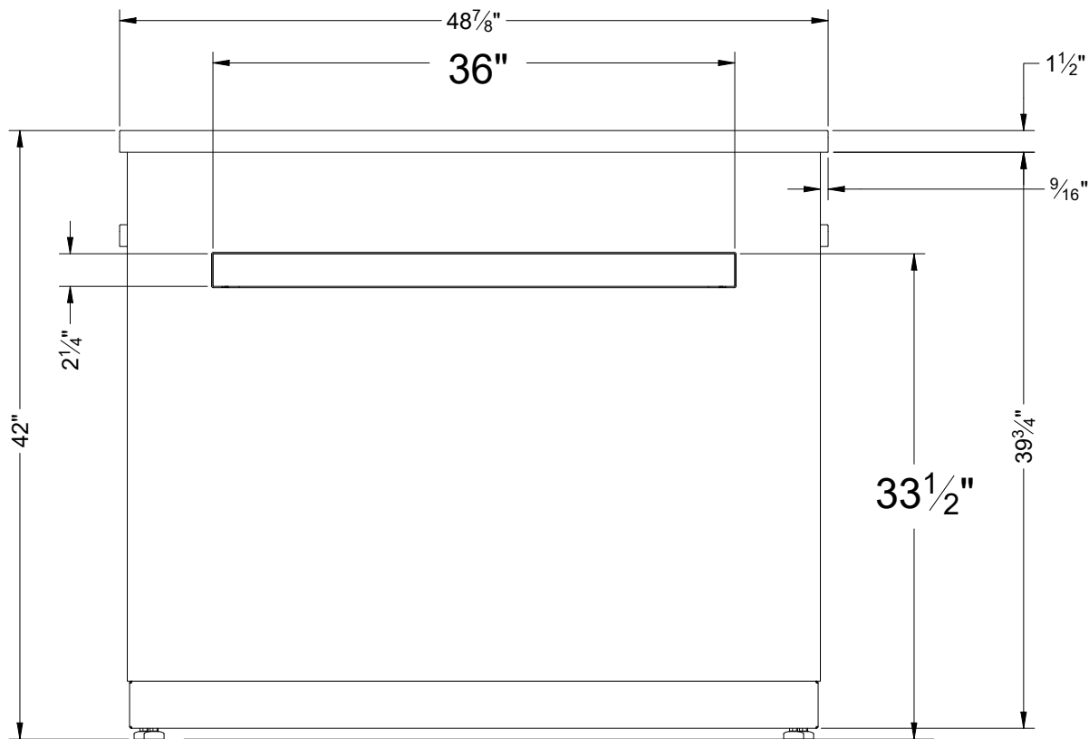
2 ELEVATION 2 SERVICE DESK
