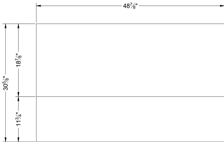
1 PLAN 2 SERVICE DESK
